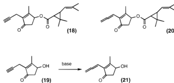
Fig. 9. A propenyl analogue of allethrin.
