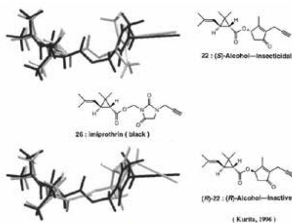
Fig. 15. Superposition of imiprothrin with prallethrin and its (R)-isomer.
