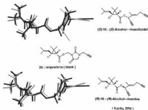
Fig. 14. Superposition of imiprothrin with (S)- and (R)-propargyl analogue of cenprothrin. (Kurita, 1996)
