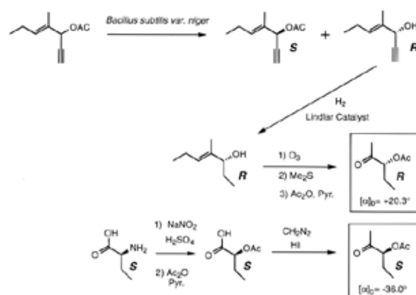
Fig. 6. Synthesis of optically active empenthrin alcohol (Matsuo 1980).
